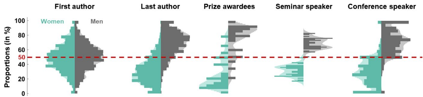
FIGURE 1 Histogram of proportions (in percentage) of women (green) and men (gray) in different aspects of neuroscientific academic life: first and last journal authors ( n = 1,760 , considering 176 journals over 10 years: 2009–2018), prize awardees ( n = 23 ), seminar speakers ( n = 38 , considering 8 seminars over the academic years 2012 to 2016), and conference speakers as invited or contributed talks ( n = 295 conferences between 2015 and 2018)
