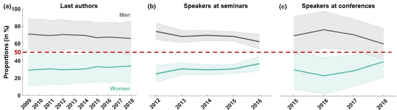
FIGURE 2 Proportions in percentage of women (green) and men (gray) as (a) last authors of journal papers (Wilcoxon rank sum test comparing 2009, n = 176 , to 2018, n = 176 : p = 0.0152 ), (b) invited speakers in seminar series (comparing 2012, n = 6 , to 2016, n = 8 : p = 0.0293 ), and (c) speakers (invited or contributed) at conferences over the years (comparing 2015, n = 30 , to 2018, n = 108 : p = 0.0062 ). Plots represent averages with \pm 1 standard deviation
